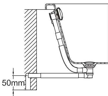
墙排式排水 Drainage through the wall
