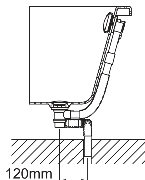
地排式排水 Drainage through the floor
